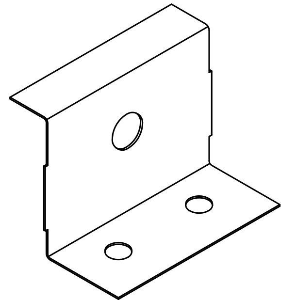
ISO VIEW SCALE 1:1
