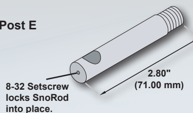
SnoPost
