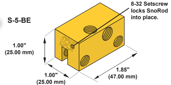
SnoPost BE
