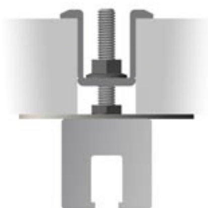
Field Condition [diagram B]
