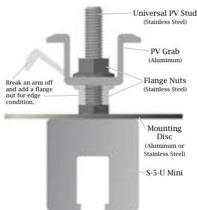
End/Edge Condition [diagram A]
